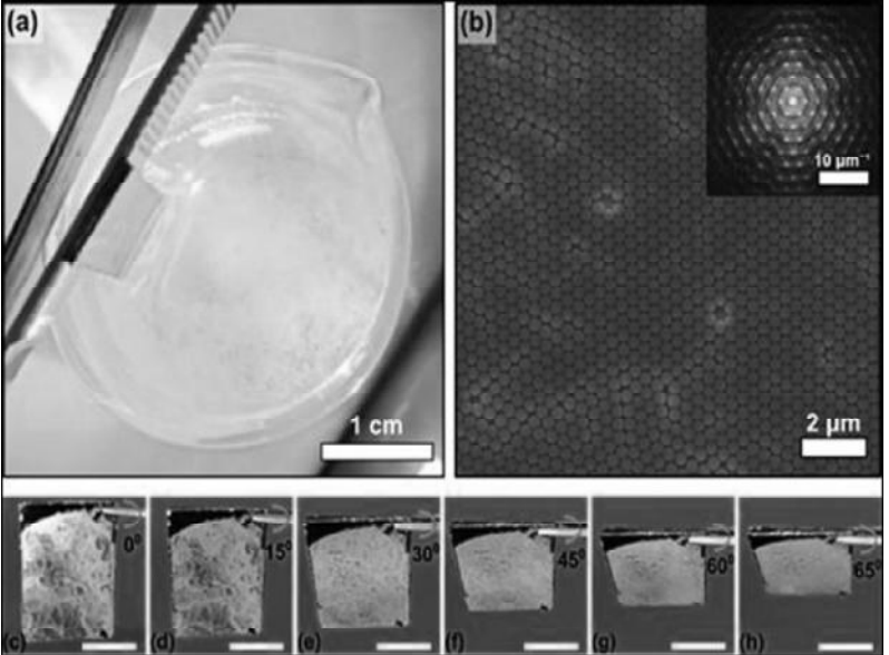
Fig: (a) Structural colors exhibited by a monolayer of PS spheres ( d_{ini} = 401 \text{ nm} ) self-assembled at the A-W interface into a hexagonally ordered close-packed (CP) state. (b) Field emission scanning electron microscope image of PS monolayer in the CP state, inset shows FFT of the image. (c-h) Structural colors exhibited by the self-assembled PS spheres for different tilt angles. The scale bar represents 0.5 \mu\text{m} (c-h).
